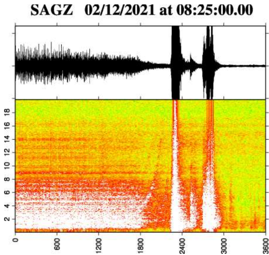
Figure S1: Spectrograms between 0 and 20 Hz for the seismic signal recorded at the vertical component of SAGA station starting at 8:25 on December 2, for a one hour duration. A gliding of the dominant spectral peak is observed between seconds 1800 and 2100, preceding the explosions starting around second 2200.
