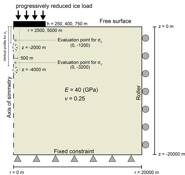
Figure 1: Axisymmetric Finite Element Method model of a pressurized shallow magma body beneath a glacier undergoing progressive unloading. The glacial load is applied as a vertical pressure over a circular area with radius r = 2500 or 5000 m, representing glaciers of different spatial extent. The unloading is implemented in incremental stages, corresponding to successive fractions of ice-thickness loss. A constant magma overpressure ( p_0 ) of 5, 10 or 20 MPa is applied to the boundary of a spherical body of 500 m radius and centred at 2000 m and 4000 m depth, embedded in a linear elastic crust (20 km-deep and 40 km-wide) with Young's Modulus E = 40 GPa and Poisson's ratio \nu = 0.25 . The minimum principal stress ( \sigma_3 ) is evaluated above the magma body at 1200 m and 3200 m depth and along a vertical profile from the surface to the top of the body. Boundary conditions include a fixed base, roller lateral boundary, and a free surface.
