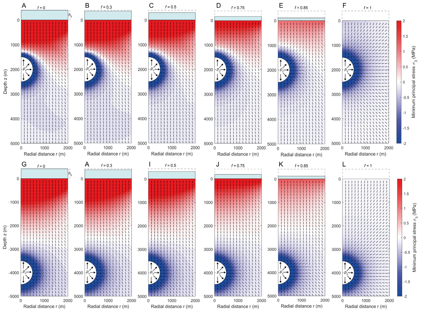
Figure 3: Minimum principal stress field ( \sigma_3 , colour scale) and orientation of the maximum principal stress ( \sigma_1 , black lines) for three scenarios with identical initial glacier geometry ( h_0 = 750 m, r = 2500 m) and magma overpressure p_0 = 10 MPa from a magma body centred at 2 km [A-F] and 4 km depth [G-L]. The parameter f is the dimensionless thinning parameter and the corresponding fraction of ice thickness removed is f^2 . [A] f = 0 , [B] f = 0.3 , [C] f = 0.5 , [D] f = 0.75 , [E] f = 0.85 , and [F] f = 1 . The initial ice thickness h_0 is indicated as a dashed line, and the remaining ice is shaded in light blue. The magma body is shown as a white circle.
