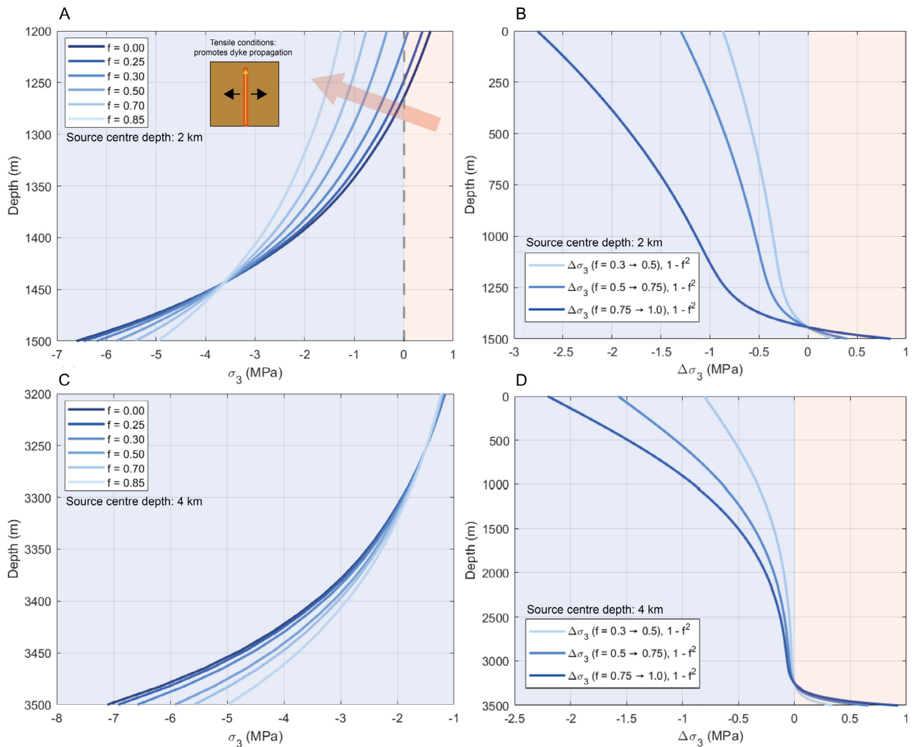
Figure 5: [A,C] Vertical profiles of the minimum principal stress ( \sigma_3 ) evaluated 300 m above a pressurized magma body for progressive glacial unloading ( f = 0-1 ), assuming an elastic crust and a constant magma overpressure of 10 MPa. Panels [A] and [C] correspond to pressure source centre depths of 2 km and 4 km, respectively. Background shading indicates compressive ( \sigma_3 > 0 , red) and tensile ( \sigma_3 < 0 , blue) stress regimes. The red arrow schematically indicates the direction of stress evolution associated with progressive glacier unloading, highlighting the transition from compressive to tensile conditions. Inset illustrate conceptual dyke trajectories under tensile stress regime. [B,D] Depth profiles of the incremental change in minimum principal stress ( \Delta\sigma_3 ) between successive stages of glacier thinning for the same configuration shown in [A] and [C]. Solid lines correspond to a quadratic unloading trajectory (proportional to 1 - f^2 ). Three unloading intervals are shown for each case: f = 0.3-0.5 , f = 0.5-0.75 , and f = 0.75-1 . Under this trajectory the three intervals remove 16%, 19% and 56% of the initial ice thickness, respectively, so that the larger late-stage \Delta\sigma_3 reflects the greater unloading within that interval rather than a non-linear mechanical response.
