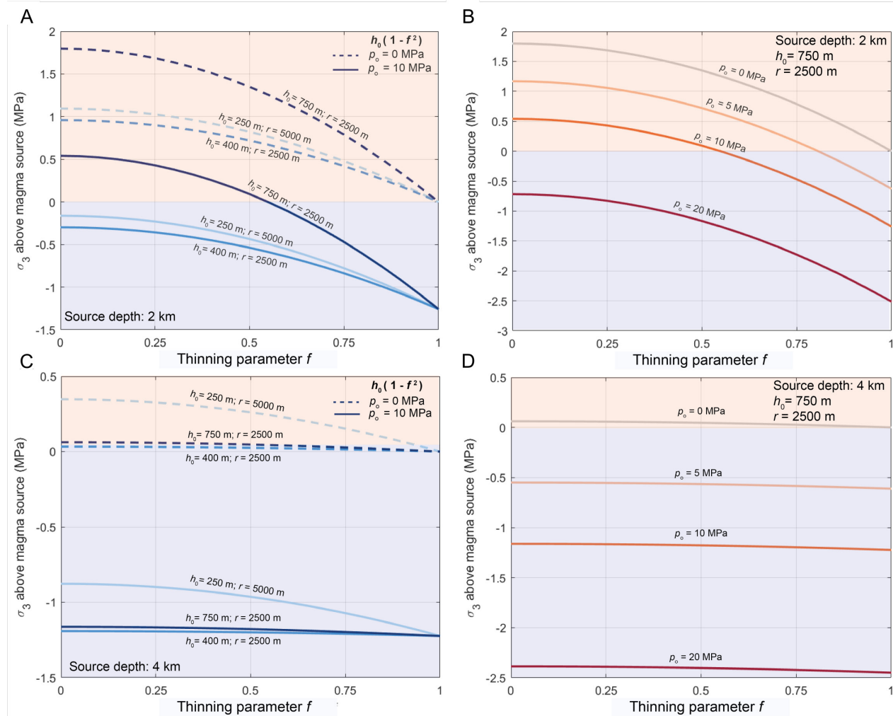
Figure 4: Evolution of the minimum principal stress ( \sigma_3 ) 300 m above a pressurized magma body as a function of the thinning parameter f , under varying glacier geometries and magma overpressure ( p_0 ) scenarios. Background shading indicates compressive ( \sigma_3 > 0 , red) and tensile ( \sigma_3 < 0 , blue) stress regimes. [A] Results for three initial ice thicknesses ( h_0 = 250, 400, 750 m), paired with glacier radii of 5000, 2500, and 2500 m, respectively, with magma overpressure p_0 = 0 MPa (dashed lines) and p_0 = 10 MPa (solid lines). Blue tones darken with increasing ice thickness. All curves correspond to a quadratic unloading trajectory, proportional to 1 - f^2 . [B] Results for a fixed glacier geometry ( h_0 = 750 m, r = 2500 m) under varying levels of magma overpressure ( p_0 = 0, 5, 10, 20 MPa), highlighting the increasingly tensile stress conditions promoted by higher internal pressurization during glacier thinning. [C–D] Same as [A–B], but for a deeper pressure source centred at 4 km.
